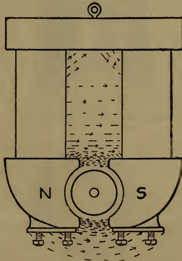
Figure 39 Magnetic leakage in bipolar dynamo, horseshoe type.
